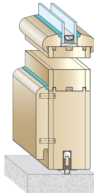
ADDITIONAL OFFER (glazing bar, weatherboard) AV-07 threshold
